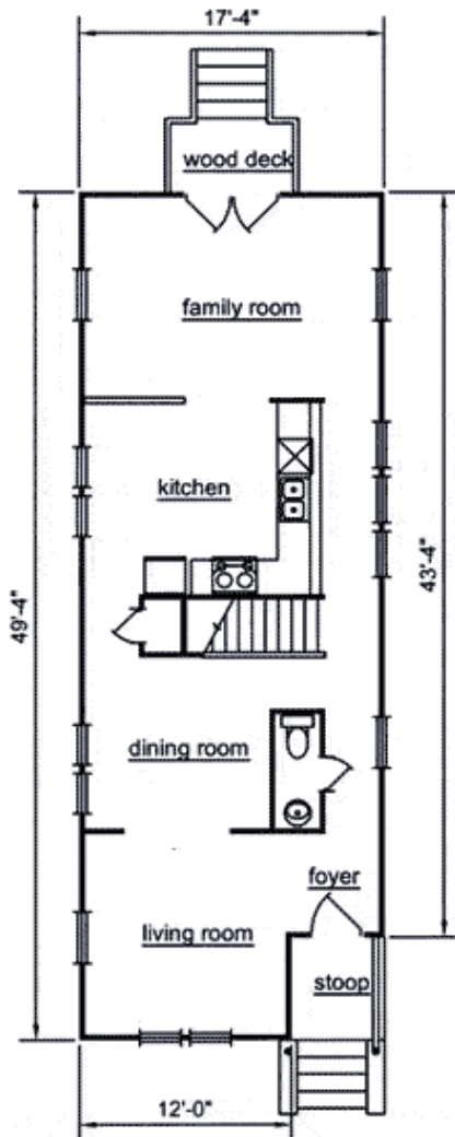
FIRST FLOOR PLAN 785 Square Feet CEIL. HT. 9'
