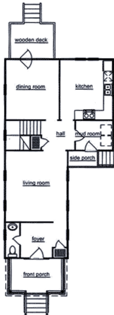
SECOND FLOOR PLAN 871 Square Feet CEIL HT. 8'
