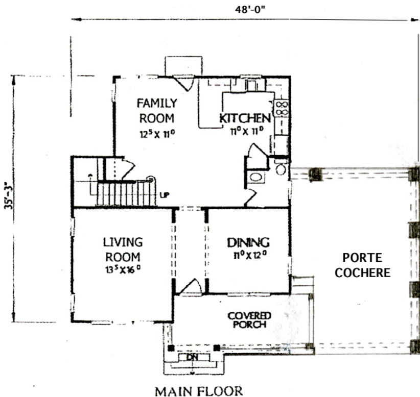
FIRST FLOOR PLAN 935 Square Feet CEIL. HT. 9'
