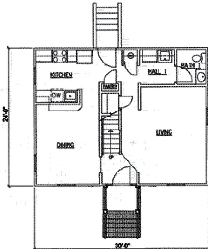
FIRST FLOOR PLAN 720 Square Feet CEIL. HT. 9'
