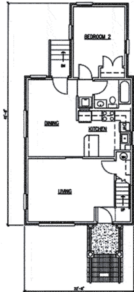
FIRST FLOOR PLAN 831 Square Feet CEIL. HT. 9'
