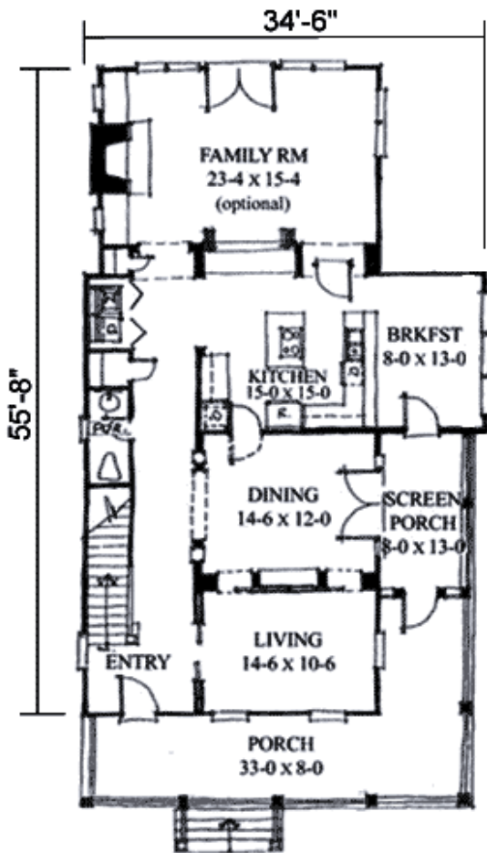
FIRST FLOOR PLAN 1463 Square Feet CEIL. HT. 9'
