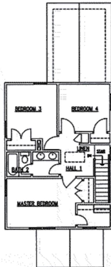
SECOND FLOOR PLAN 660 Square Feet CEIL HT. 8'
