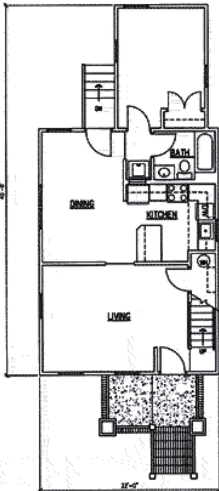
FIRST FLOOR PLAN 831 Square Feet CEIL. HT. 9'
