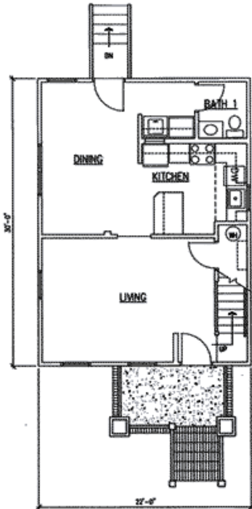
FIRST FLOOR PLAN 660 Square Feet CEIL. HT. 9'
