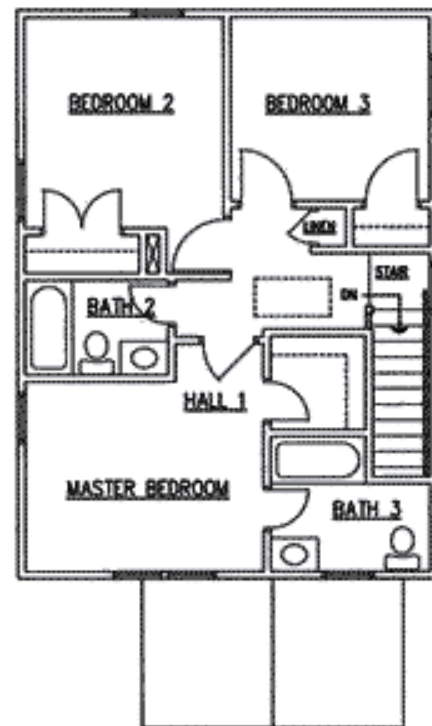
SECOND FLOOR PLAN 660 Square Feet CEIL HT. 8'
