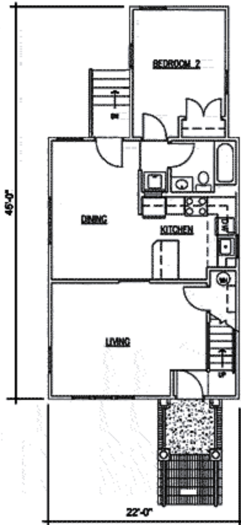
FIRST FLOOR PLAN 831 Square Feet CEIL. HT. 9'
