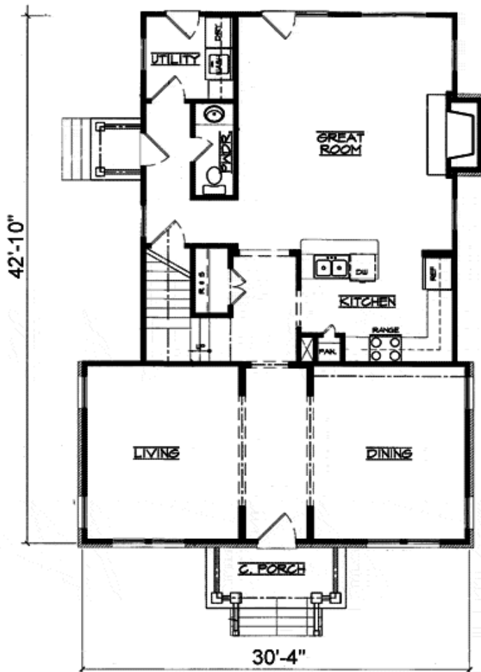
FIRST FLOOR PLAN 1178 Square Feet CEIL. HT. 9'
