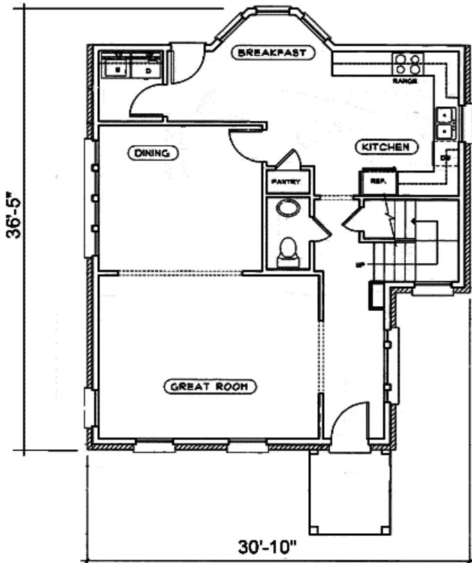
FIRST FLOOR PLAN 928 Square Feet CEIL. HT. 9'
