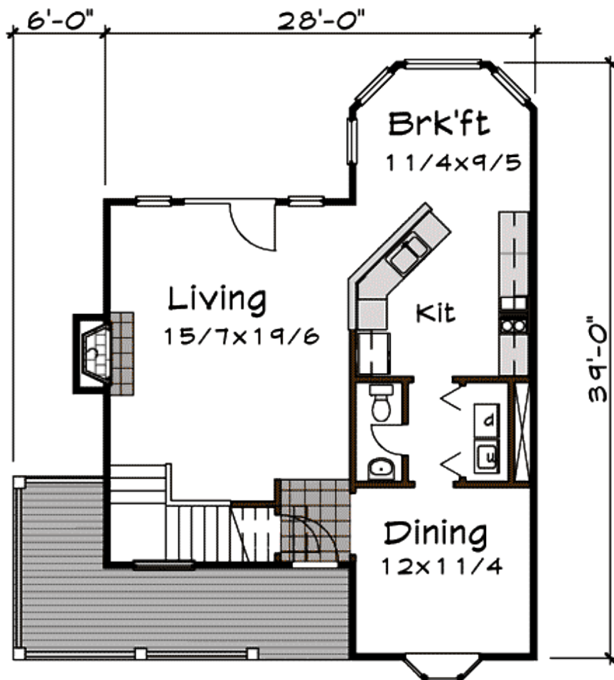
Floor 1 plan
