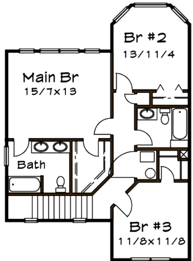
Floor 2 plan
